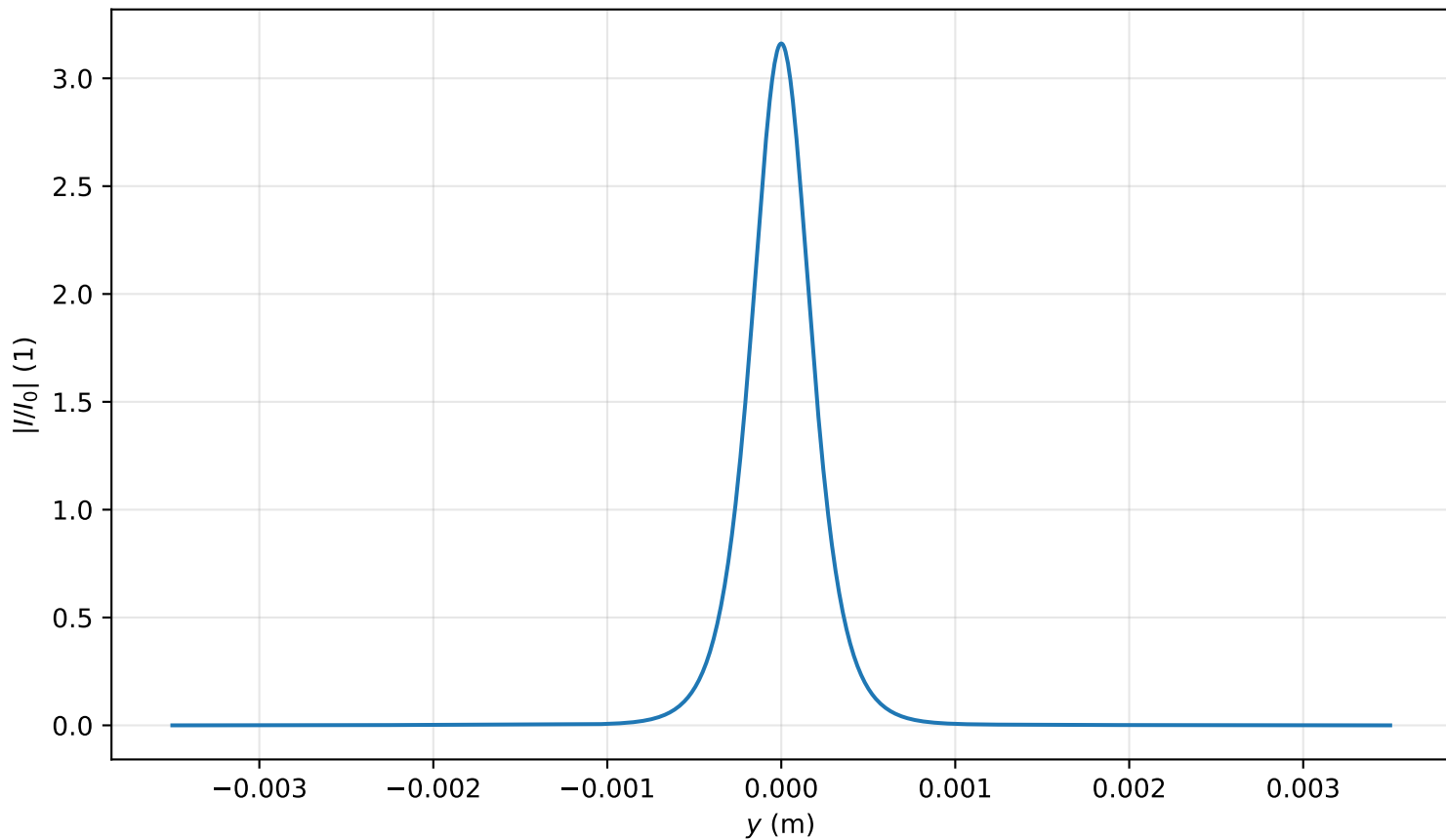
Intensity profile I(x=0, y, z=3.742)/I_0 , \text{Pin}=1.0\text{Pcr} , artificial time
